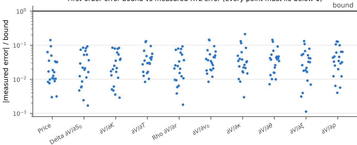
First-order error bound vs measured RTL error (every point must lie below 1)
